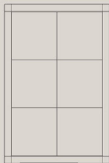
BER VIT 2 OH/MH/BH B 1166 mm / H 1810 mm / D 530 mm
