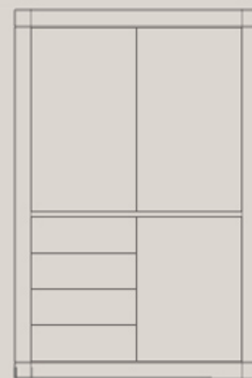
BER VIT 2 LD/BH B 1166 mm / H 1810 mm / D 530 mm
